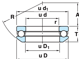
With spherical back face
